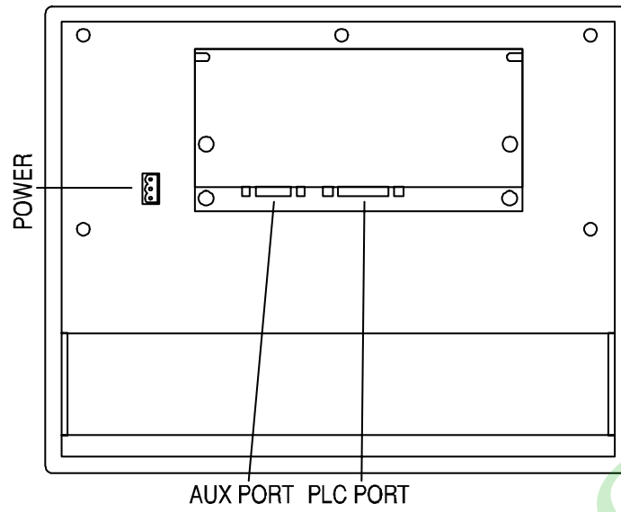
Figure 37 - Connectors
