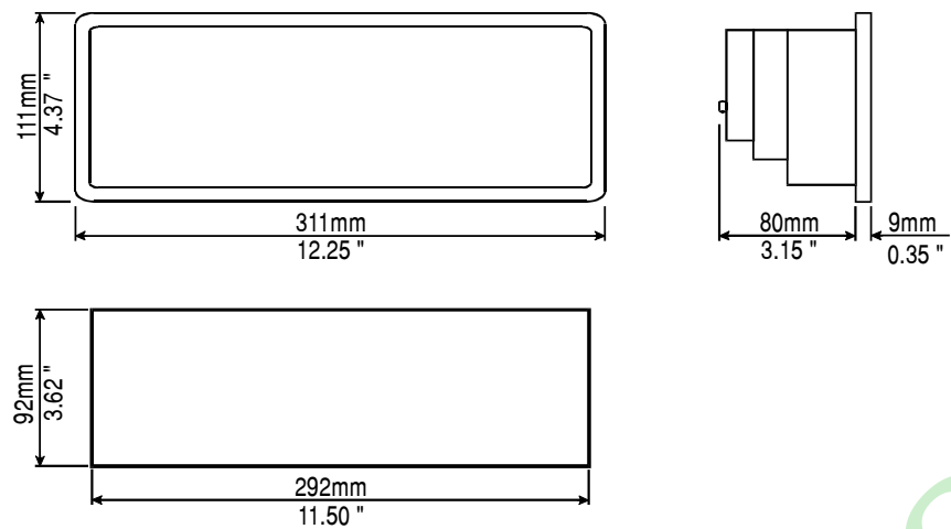
Figure 8 - Dimensions
